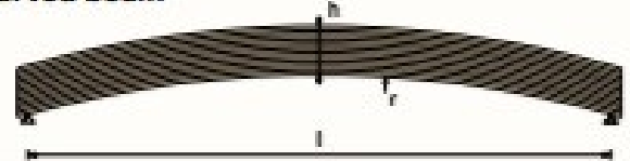
Double tapered beam with curved lower chord
