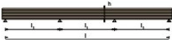
Parallel beam with structural camber
